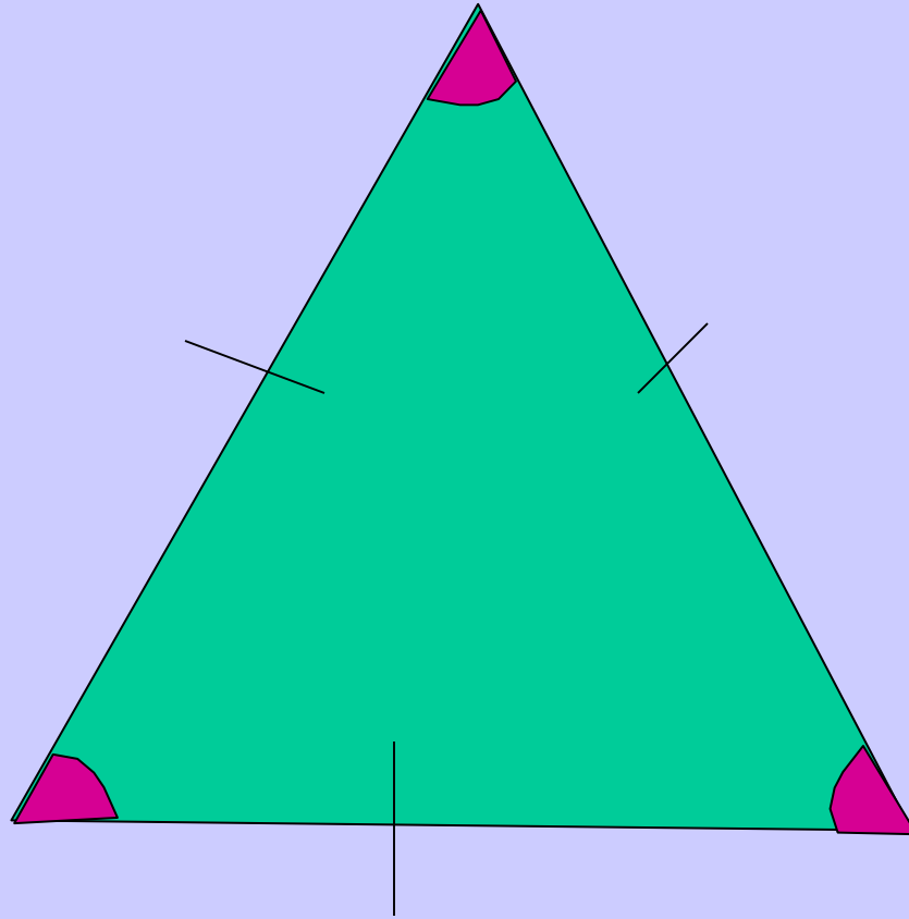
equilateral triangle
